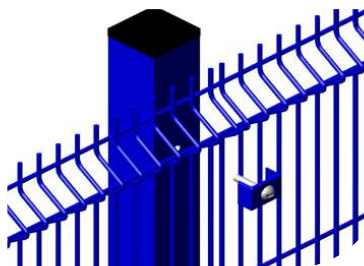
RFS Cal-Tech Steel Clip Fixing
